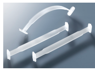
8/00 Grifflänge: 155 mm Tragkraft: max. 15kg 8/00 Handle length: 155mm. Capacity: max. 15kg.
